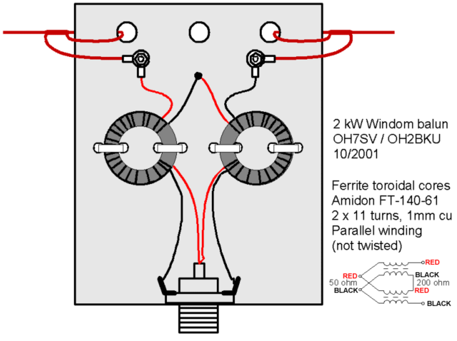
Windom balun made with Amidon ferrite toroids
