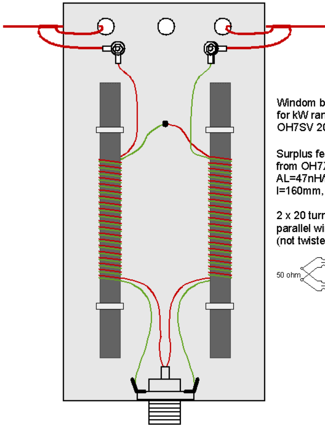
Window balun made with surplus ferrite rods
